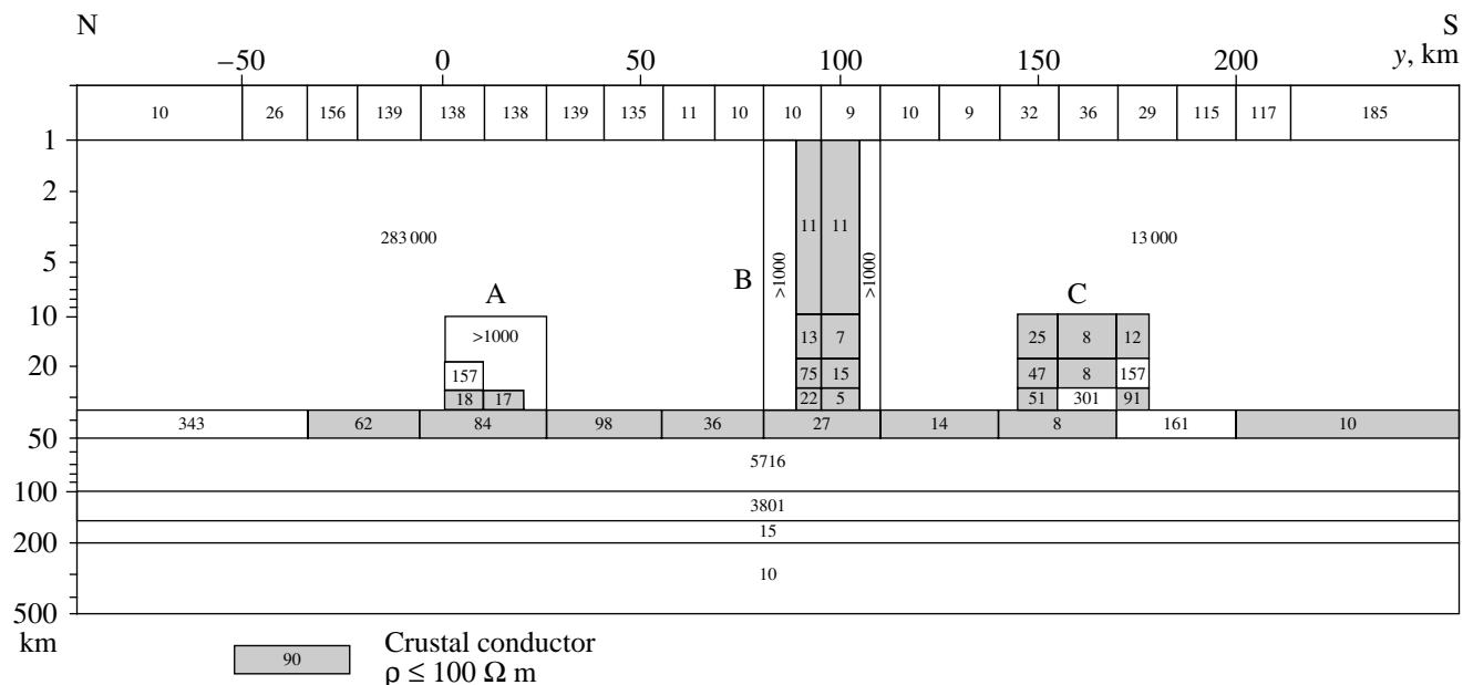
Fig. 13. The TM model: inversion of \rho^\perp and \phi^\perp using the I12DC program; resistivity values (in \Omega \text{ m} ) are shown within blocks, and the region of lower crustal resistivities is shaded (cf. Fig. 4).
