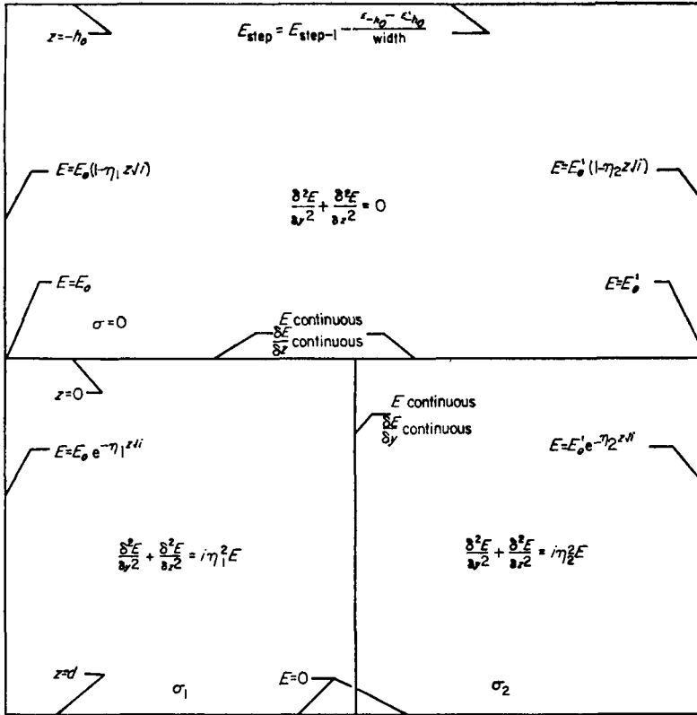
FIG. 3. E polarization. Equations and boundary conditions for E_x .
