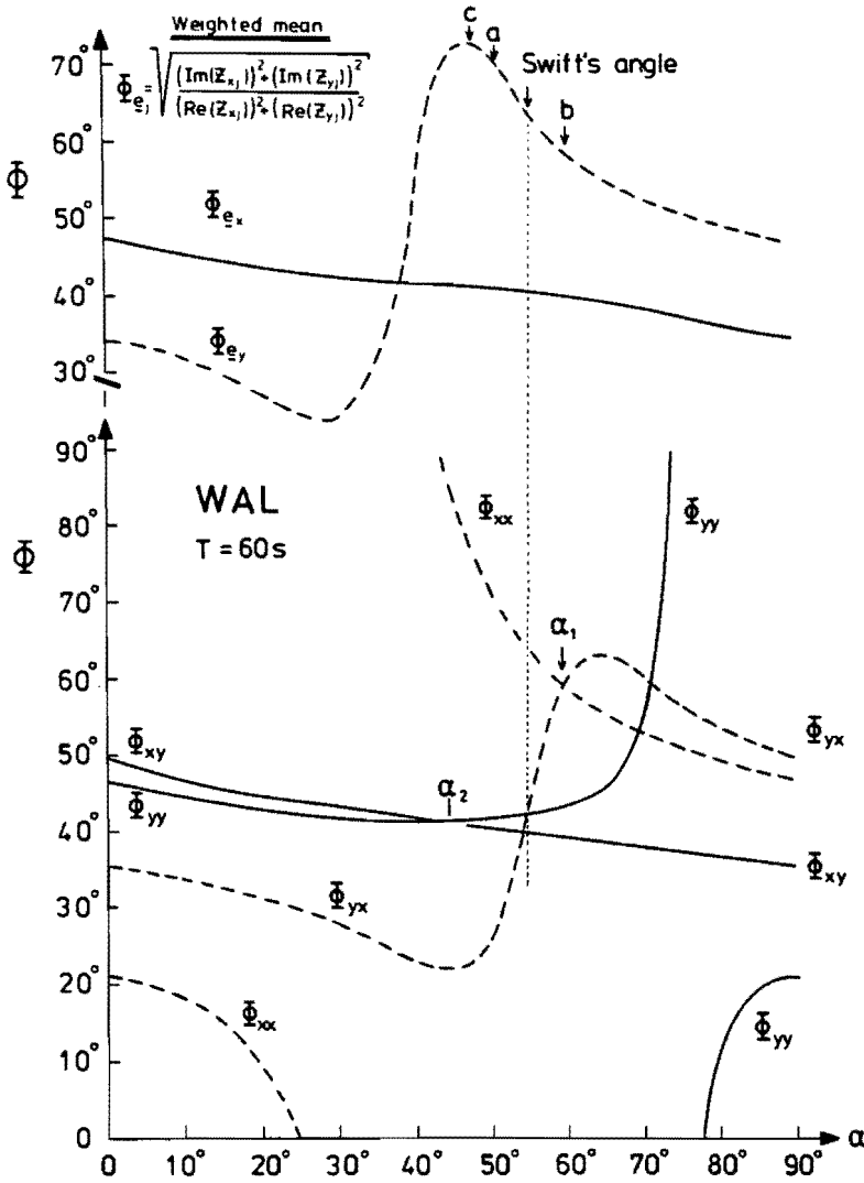
Fig. 4. Phases of the elements of the impedance tensor (bottom) and phases of the 'telluric vectors', according to Eq. (20), of site WAL, T=1 min, at a stepwise coordinate transformation. The impedances of the main diagonal elements are comparable with their confidence intervals for angles around 75^\circ and 35^\circ , and they have negative phases there. Then, it is not useful to calculate a phase according to Eq. (20) there. Elsewhere, |\Delta Z/Z| < 0.1 ( \beta = 68\% ) and |\Delta\phi| < 5^\circ ; the errors of all phases are smaller than the referred differences between \phi_{e_x} and \phi_{e_y} . For further explanation, see text
